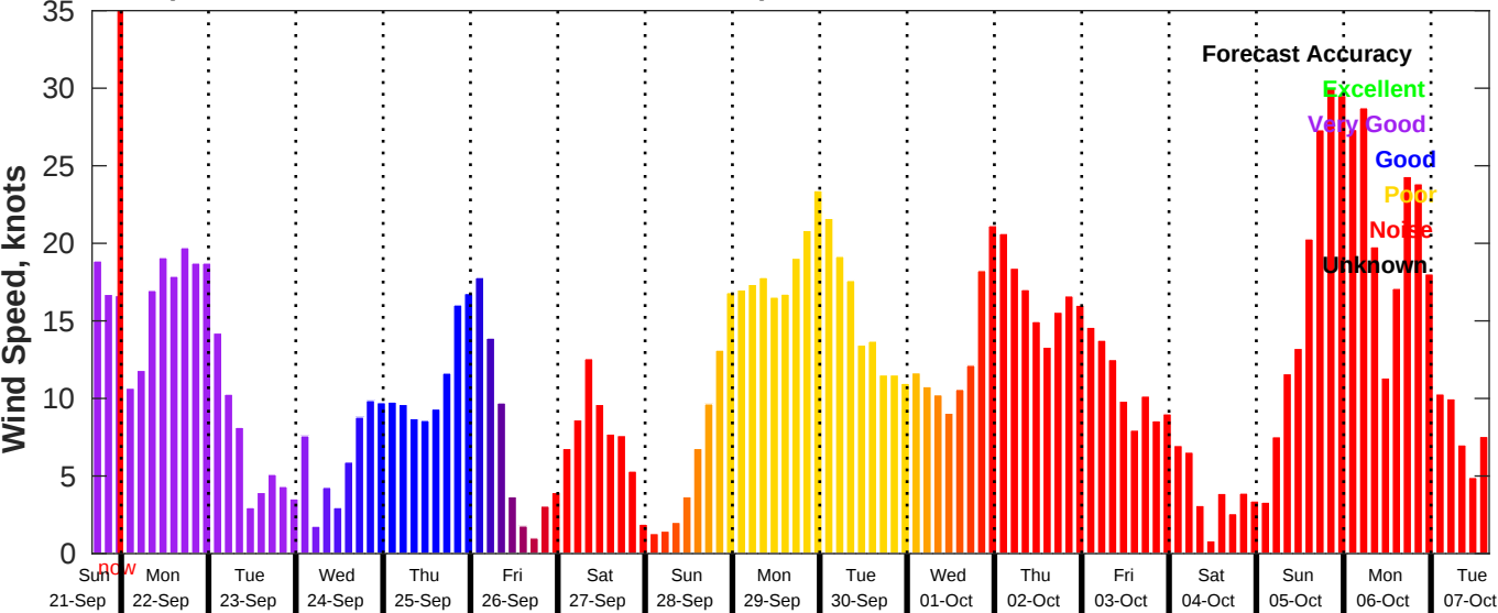
GFS Wind Speed Forecast for NDBC 46028 from 21-Sep-2025 16:00:00 to 07-Oct-2025 16:00:00
