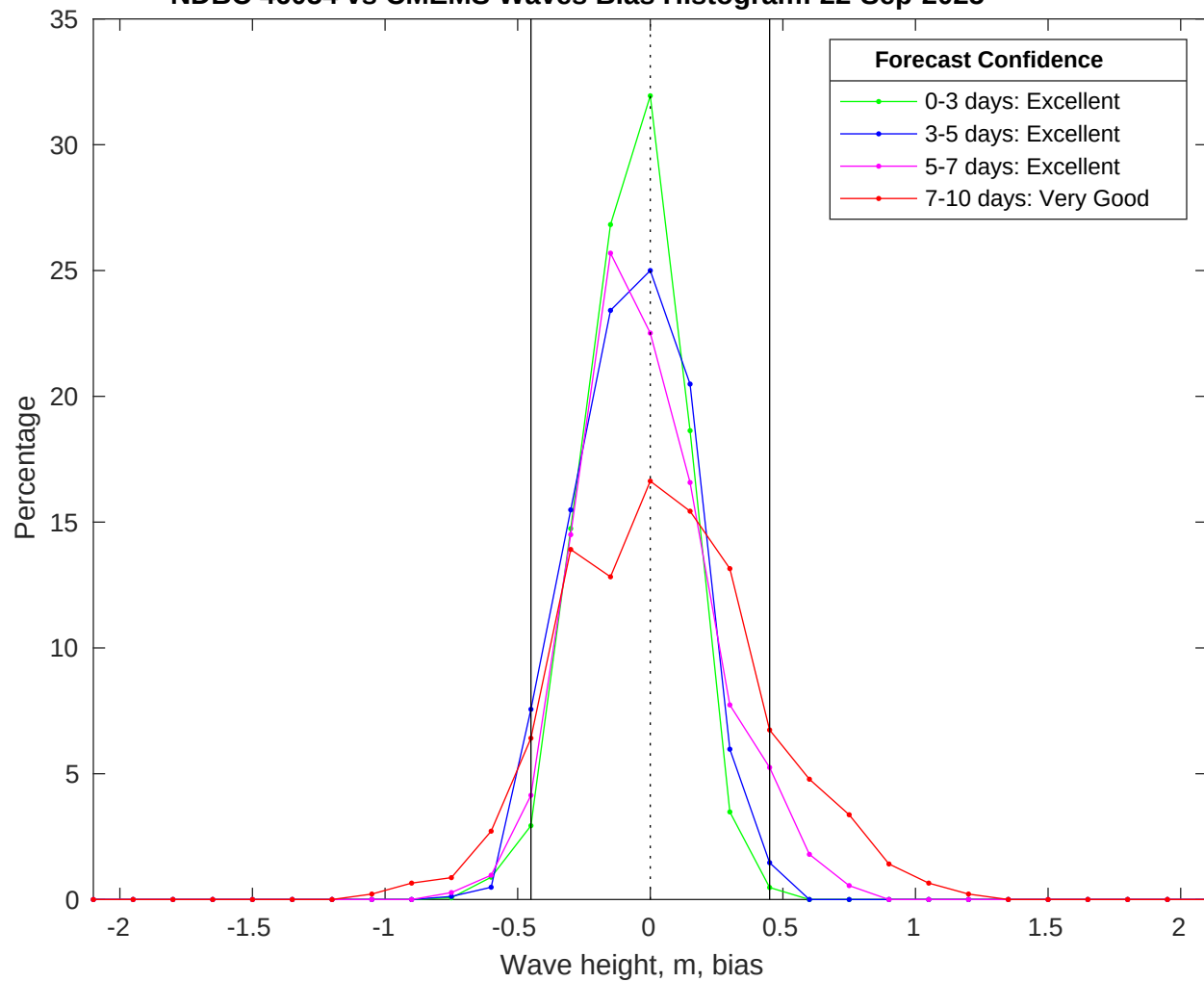
NDBC 46054 vs CMEMS Waves Bias Histogram: 22-Sep-2025
