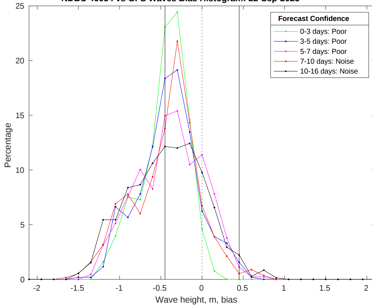
NDBC 46054 vs GFS Waves Bias Histogram: 22-Sep-2025
