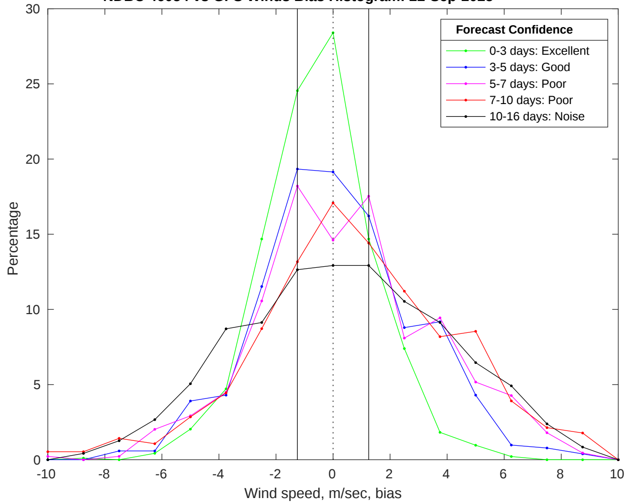
NDBC 46054 vs GFS Winds Bias Histogram: 22-Sep-2025
