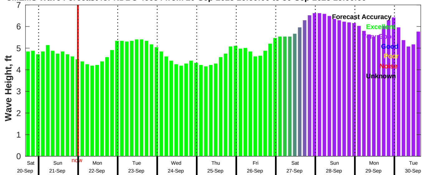
CMEMS Wave Forecast for NDBC 46054 from 20-Sep-2025 16:00:00 to 30-Sep-2025 16:00:00
