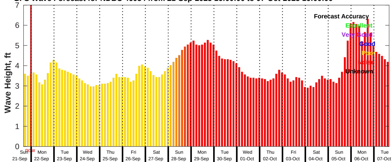
GFS Wave Forecast for NDBC 46054 from 21-Sep-2025 16:00:00 to 07-Oct-2025 16:00:00
