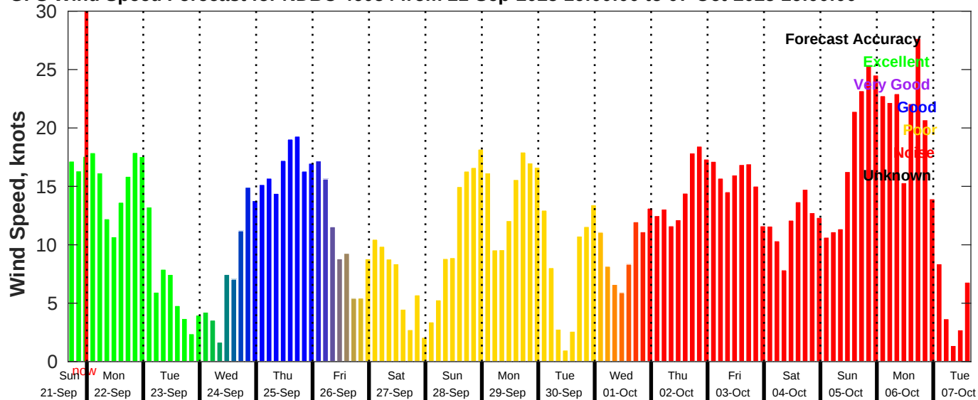
GFS Wind Speed Forecast for NDBC 46054 from 21-Sep-2025 16:00:00 to 07-Oct-2025 16:00:00
