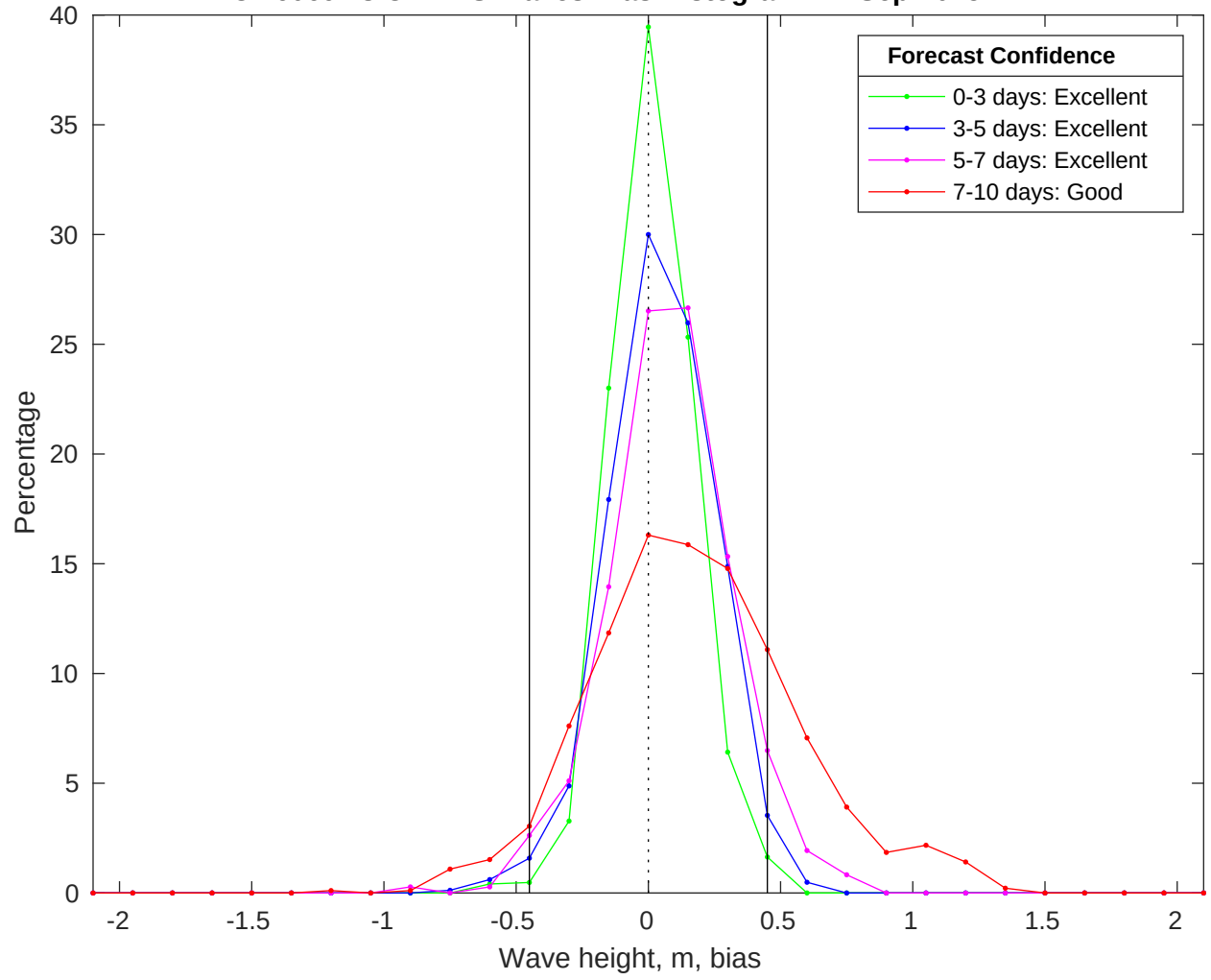
NDBC 46069 vs CMEMS Waves Bias Histogram: 22-Sep-2025
