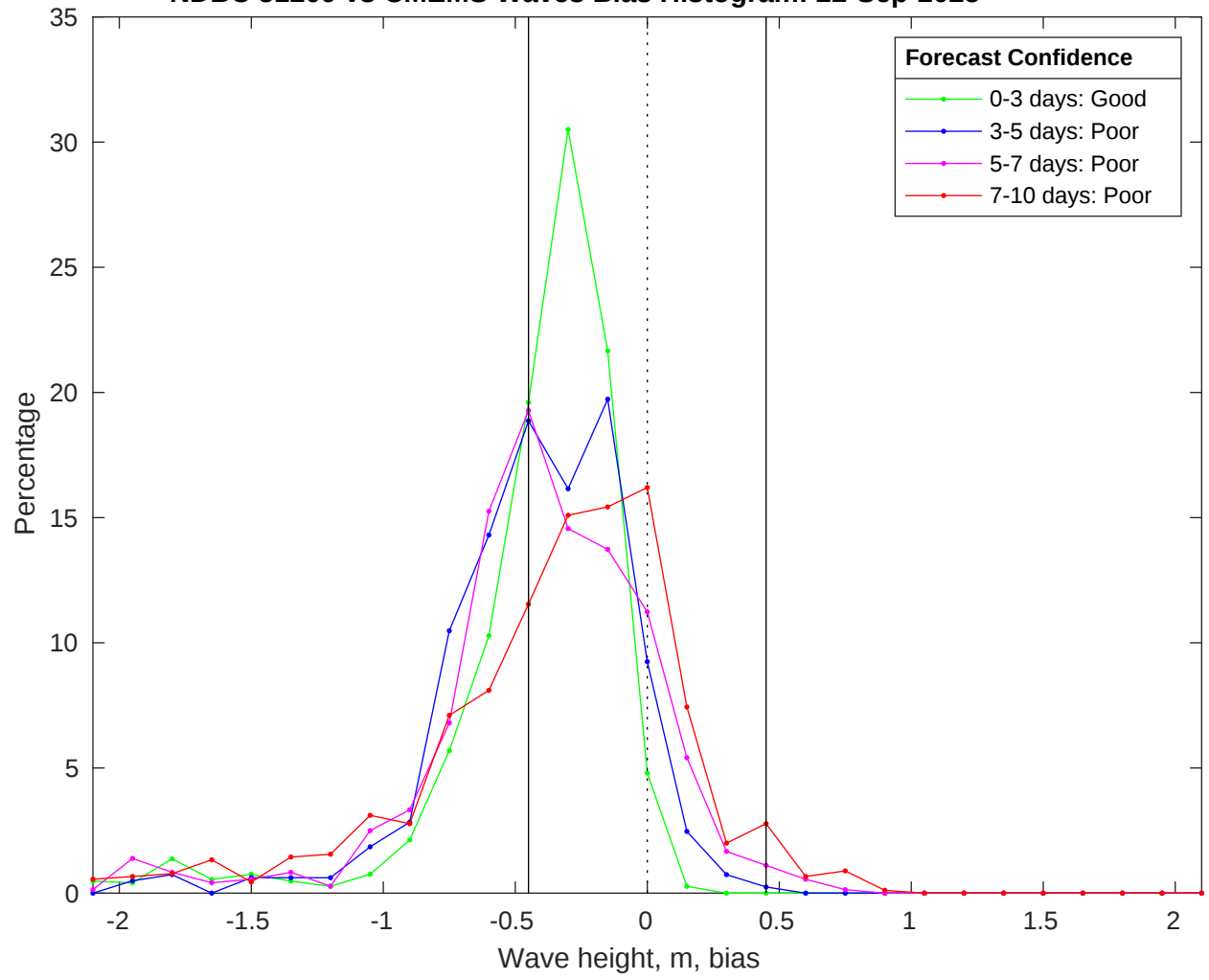
NDBC 51209 vs CMEMS Waves Bias Histogram: 22-Sep-2025
