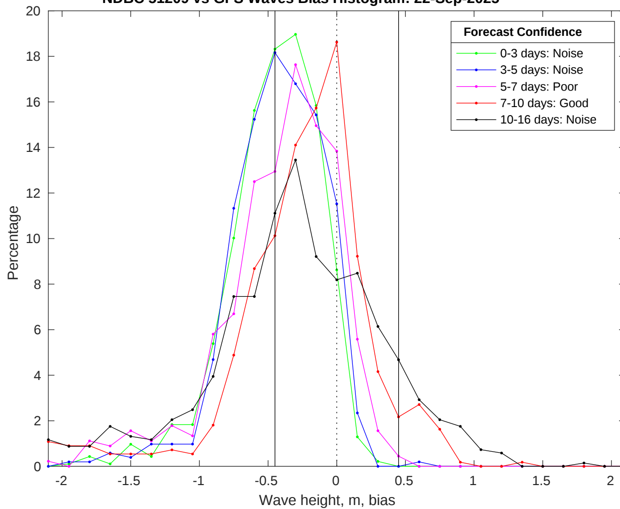
NDBC 51209 vs GFS Waves Bias Histogram: 22-Sep-2025
