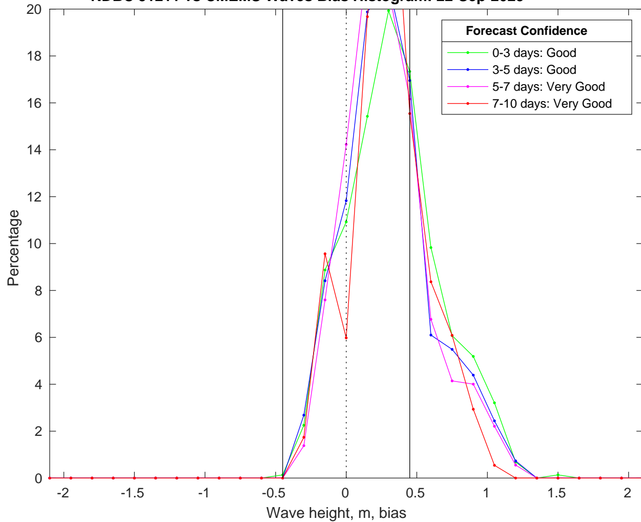
NDBC 51211 vs CMEMS Waves Bias Histogram: 22-Sep-2025
