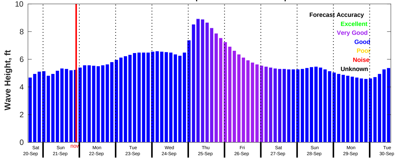
CMEMS Wave Forecast for NDBC 51211 from 20-Sep-2025 14:00:00 to 30-Sep-2025 14:00:00
