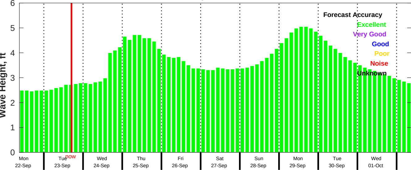
CMEMS Wave Forecast for NDBC 52212 from 21-Sep-2025 09:00:00 to 01-Oct-2025 09:00:00
