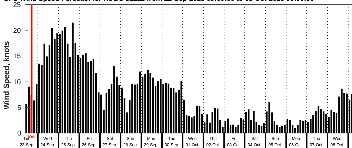
GFS Wind Speed Forecast for NDBC 52212 from 22-Sep-2025 09:00:00 to 08-Oct-2025 09:00:00
