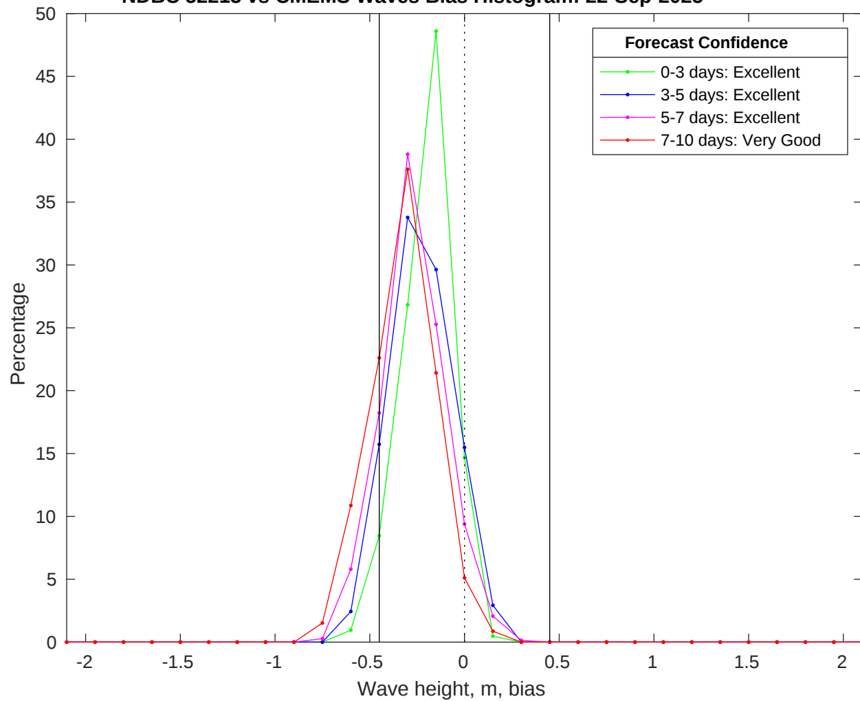
NDBC 52213 vs CMEMS Waves Bias Histogram: 22-Sep-2025
