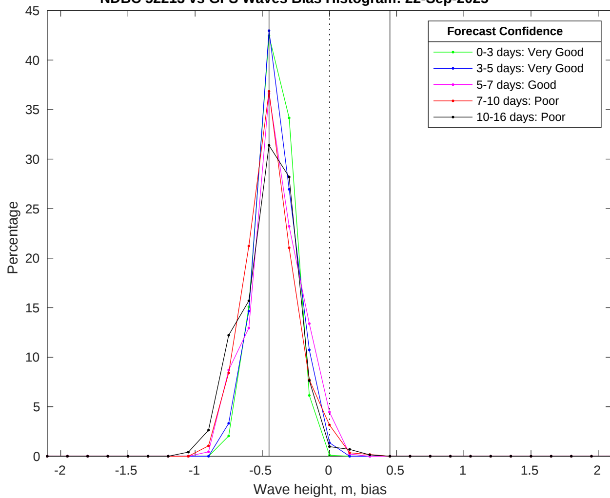
NDBC 52213 vs GFS Waves Bias Histogram: 22-Sep-2025
