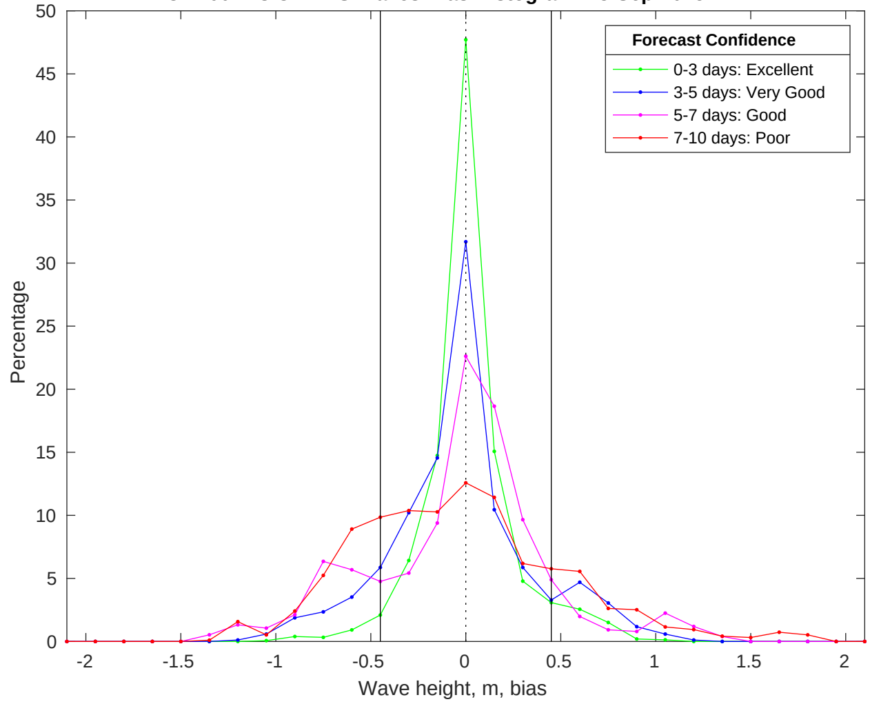
NDBC 41004 vs CMEMS Waves Bias Histogram: 23-Sep-2025
