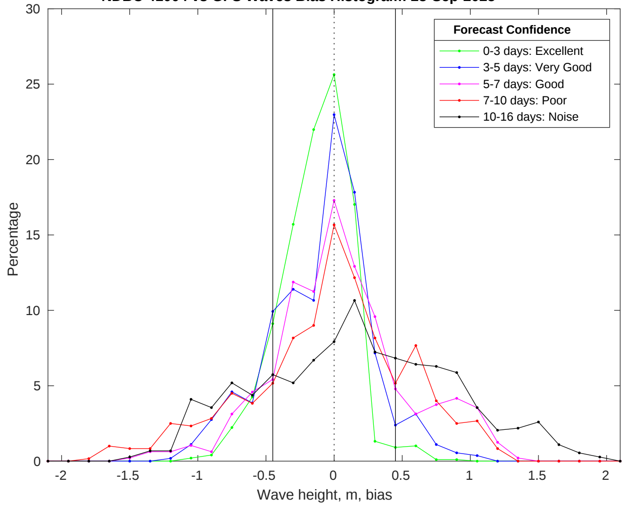
NDBC 41004 vs GFS Waves Bias Histogram: 23-Sep-2025
