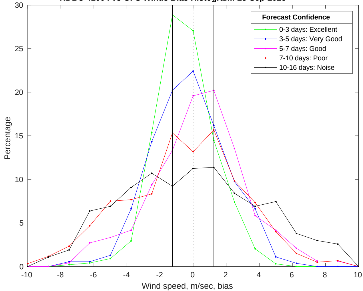
NDBC 41004 vs GFS Winds Bias Histogram: 23-Sep-2025
