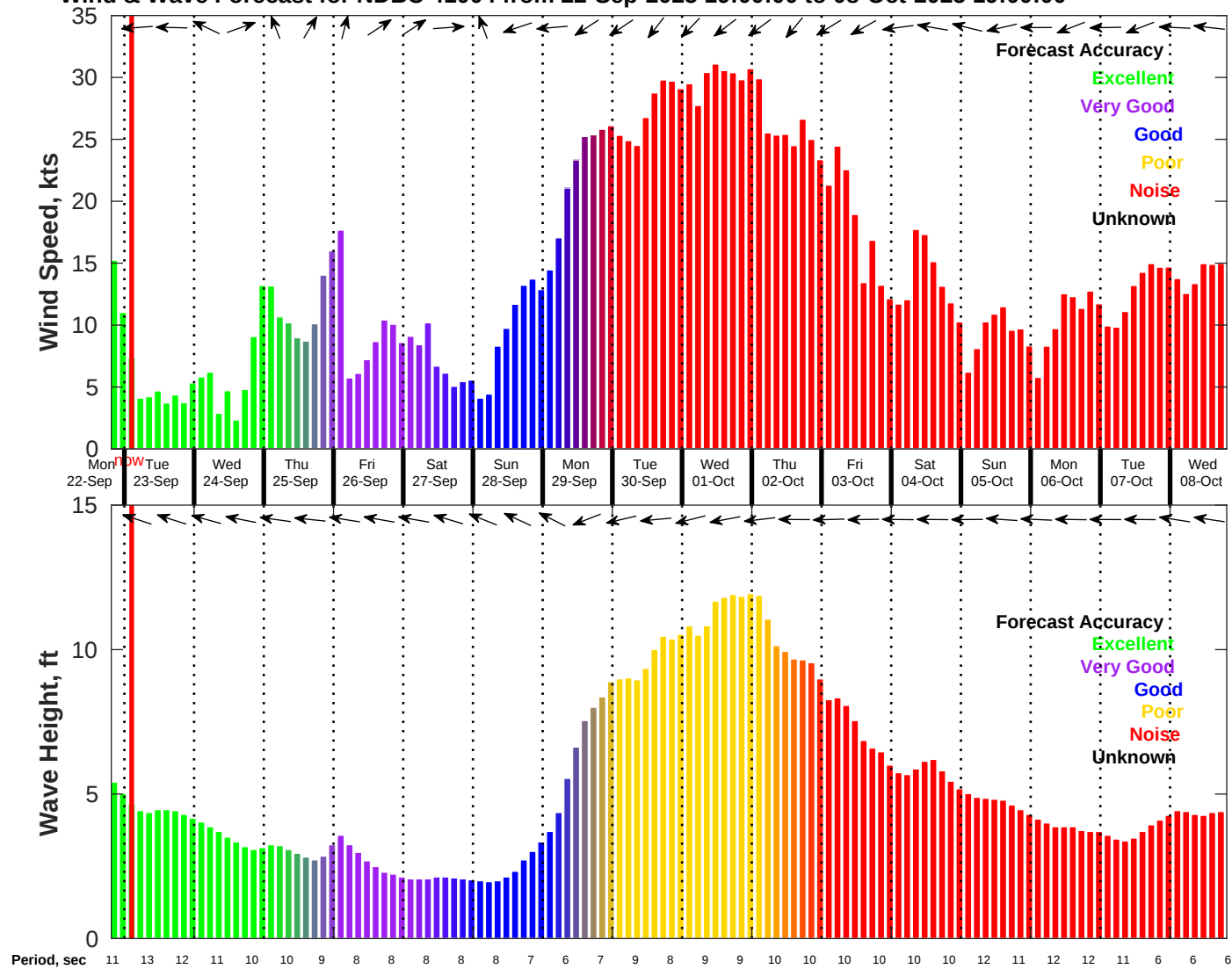
Wind & Wave Forecast for NDBC 41004 from 22-Sep-2025 19:00:00 to 08-Oct-2025 19:00:00
