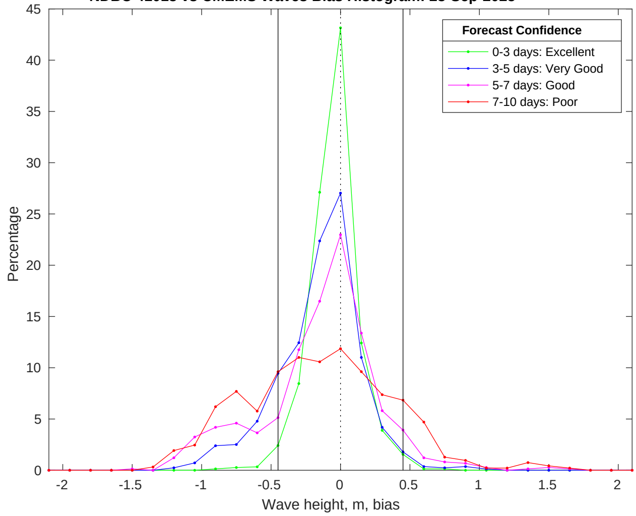
NDBC 41013 vs CMEMS Waves Bias Histogram: 23-Sep-2025
