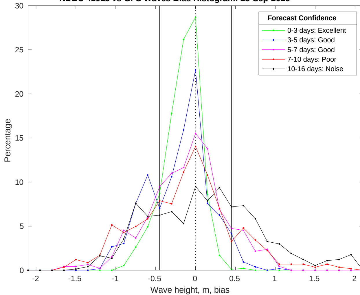
NDBC 41013 vs GFS Waves Bias Histogram: 23-Sep-2025
