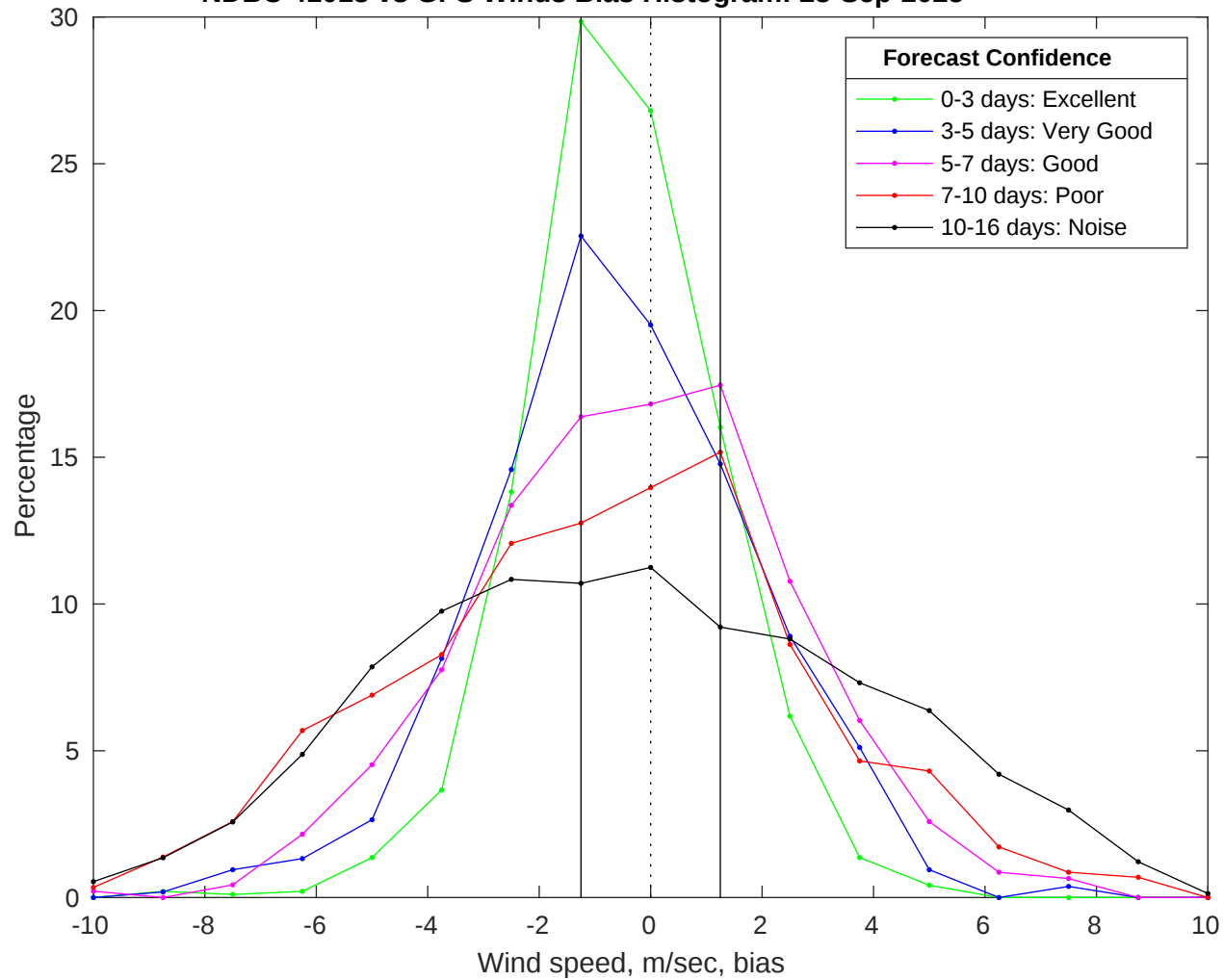
NDBC 41013 vs GFS Winds Bias Histogram: 23-Sep-2025
