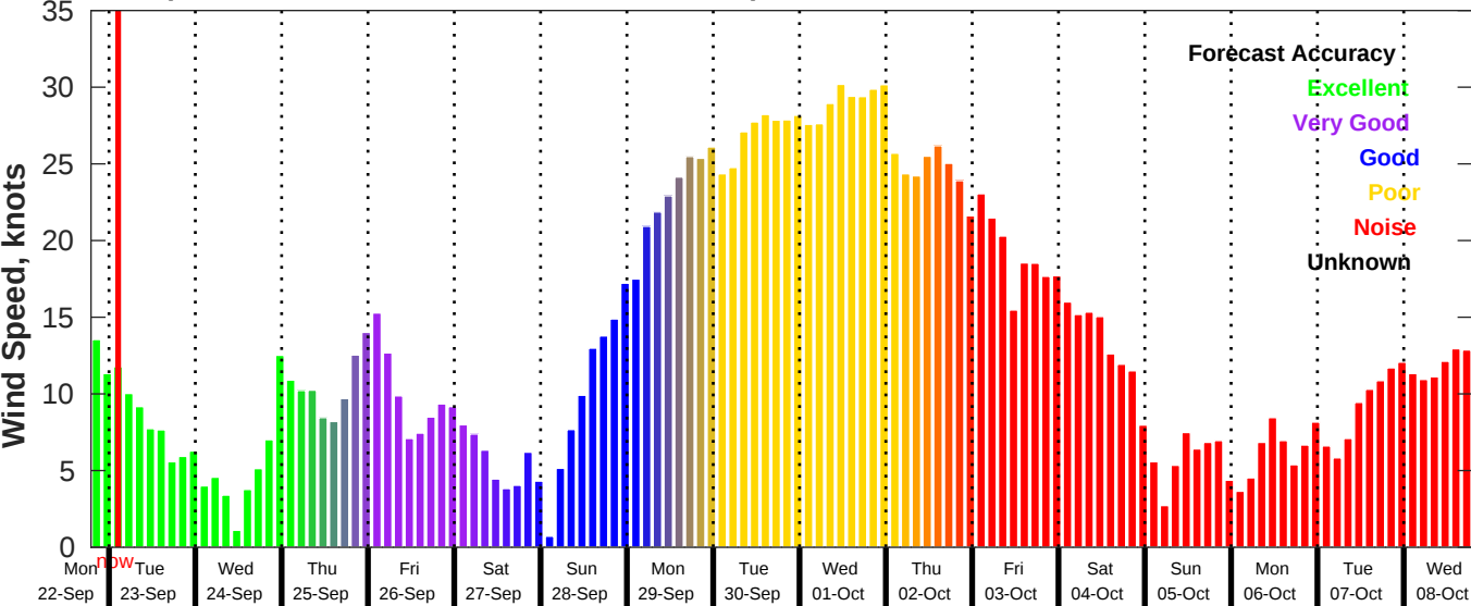
GFS Wind Speed Forecast for NDBC 41013 from 22-Sep-2025 19:00:00 to 08-Oct-2025 19:00:00
