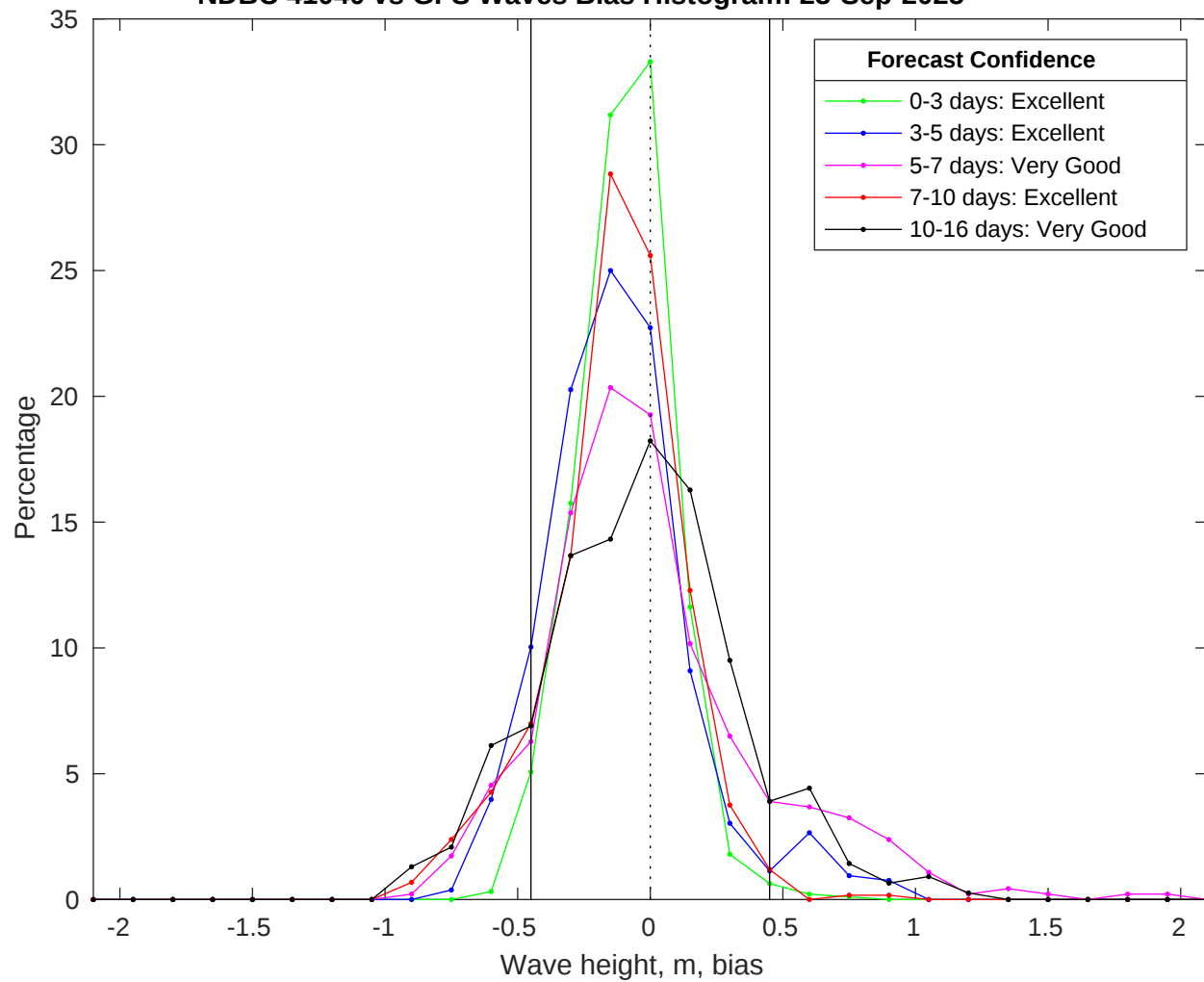
NDBC 41040 vs GFS Waves Bias Histogram: 23-Sep-2025
