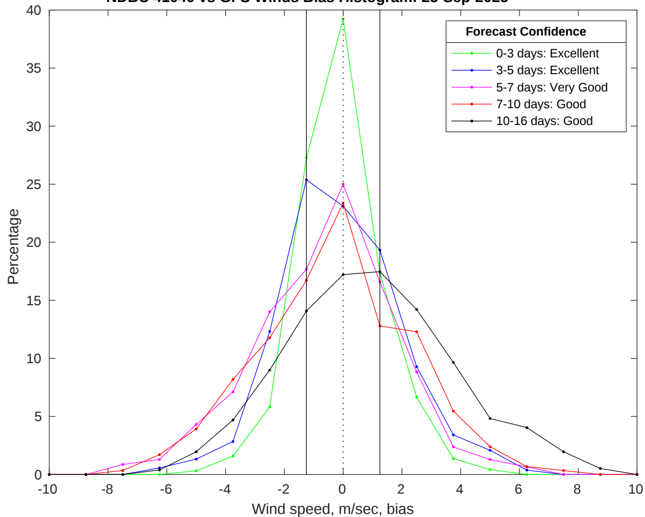
NDBC 41040 vs GFS Winds Bias Histogram: 23-Sep-2025
