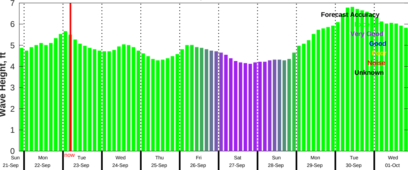
CMEMS Wave Forecast for NDBC 41040 from 21-Sep-2025 21:00:00 to 01-Oct-2025 21:00:00
