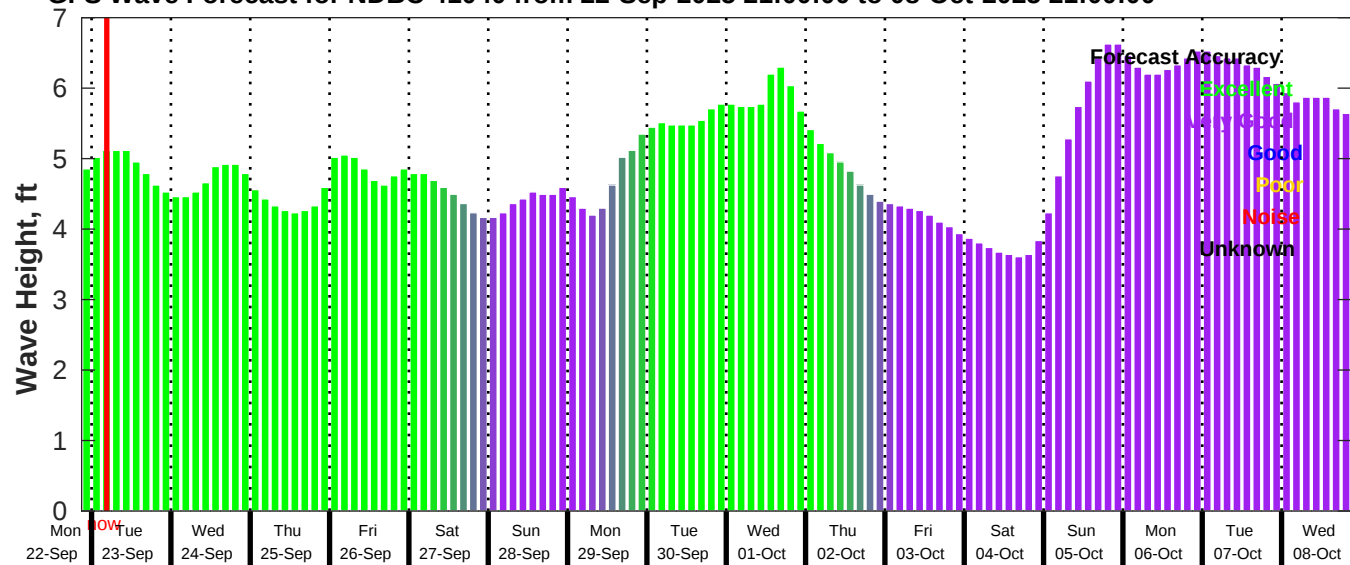
GFS Wave Forecast for NDBC 41040 from 22-Sep-2025 21:00:00 to 08-Oct-2025 21:00:00
