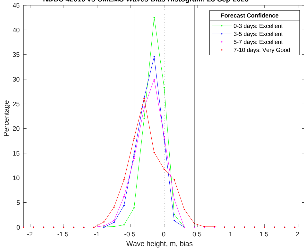
NDBC 42019 vs CMEMS Waves Bias Histogram: 23-Sep-2025
