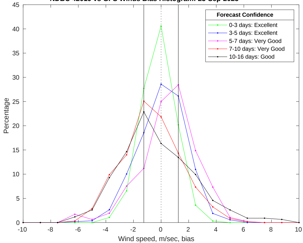
NDBC 42019 vs GFS Winds Bias Histogram: 23-Sep-2025
