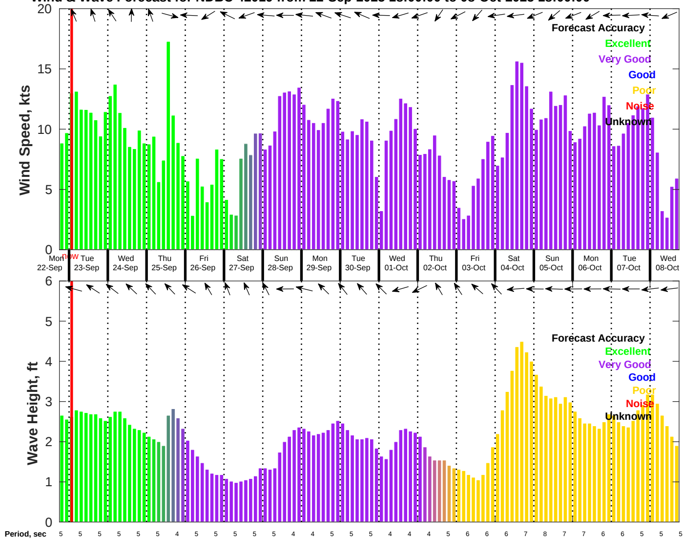
Wind & Wave Forecast for NDBC 42019 from 22-Sep-2025 18:00:00 to 08-Oct-2025 18:00:00
