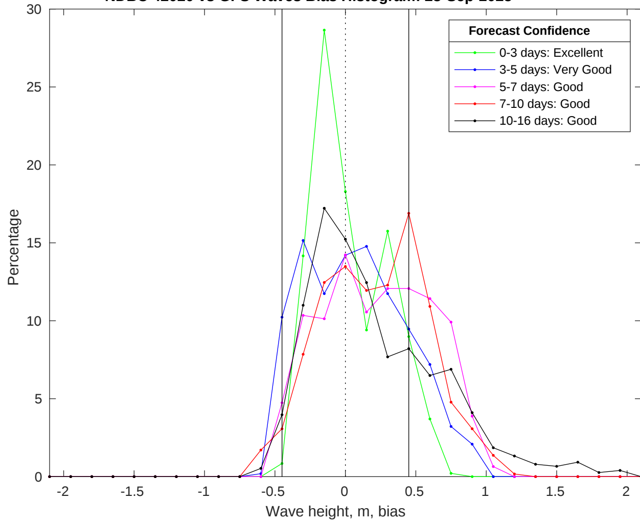
NDBC 42020 vs GFS Waves Bias Histogram: 23-Sep-2025
