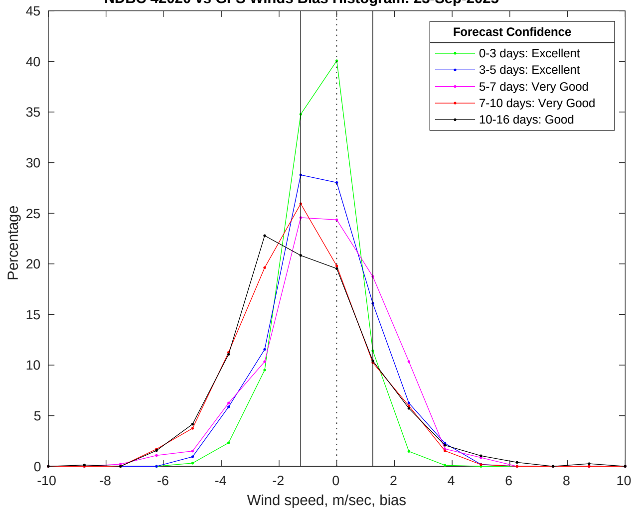
NDBC 42020 vs GFS Winds Bias Histogram: 23-Sep-2025
