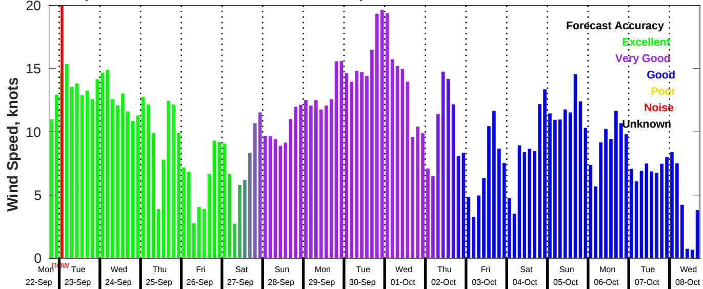
GFS Wind Speed Forecast for NDBC 42020 from 22-Sep-2025 18:00:00 to 08-Oct-2025 18:00:00
