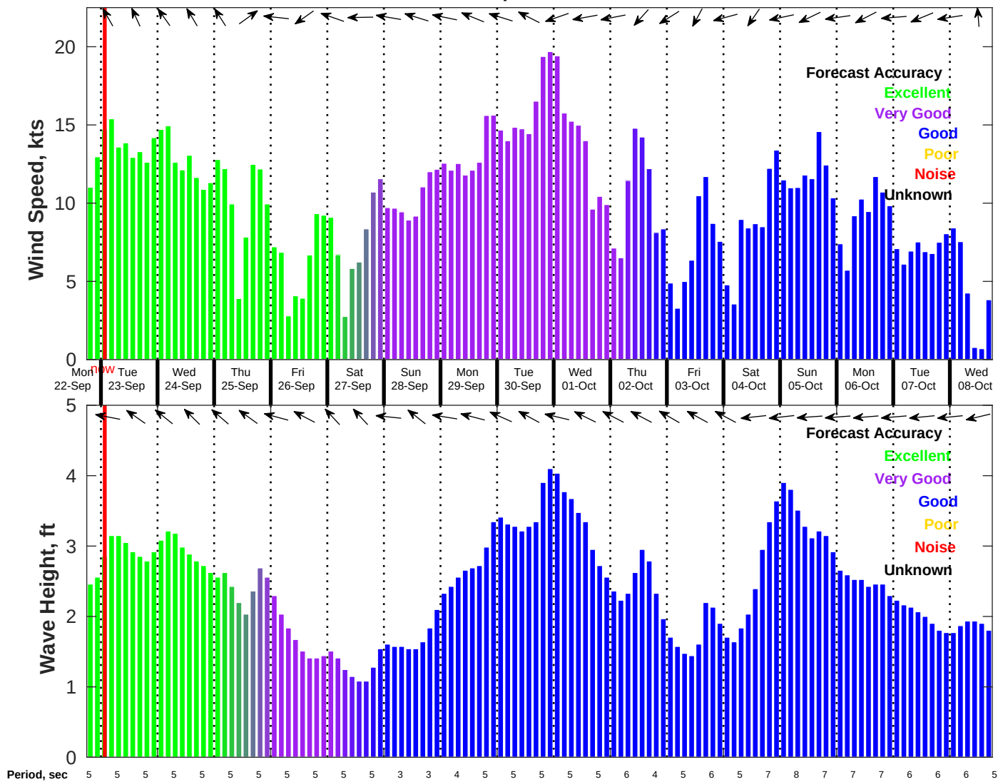
Wind & Wave Forecast for NDBC 42020 from 22-Sep-2025 18:00:00 to 08-Oct-2025 18:00:00
