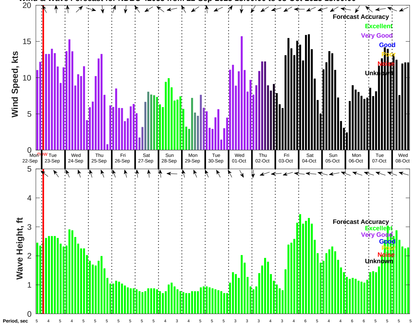
Wind & Wave Forecast for NDBC 42035 from 22-Sep-2025 18:00:00 to 08-Oct-2025 18:00:00
