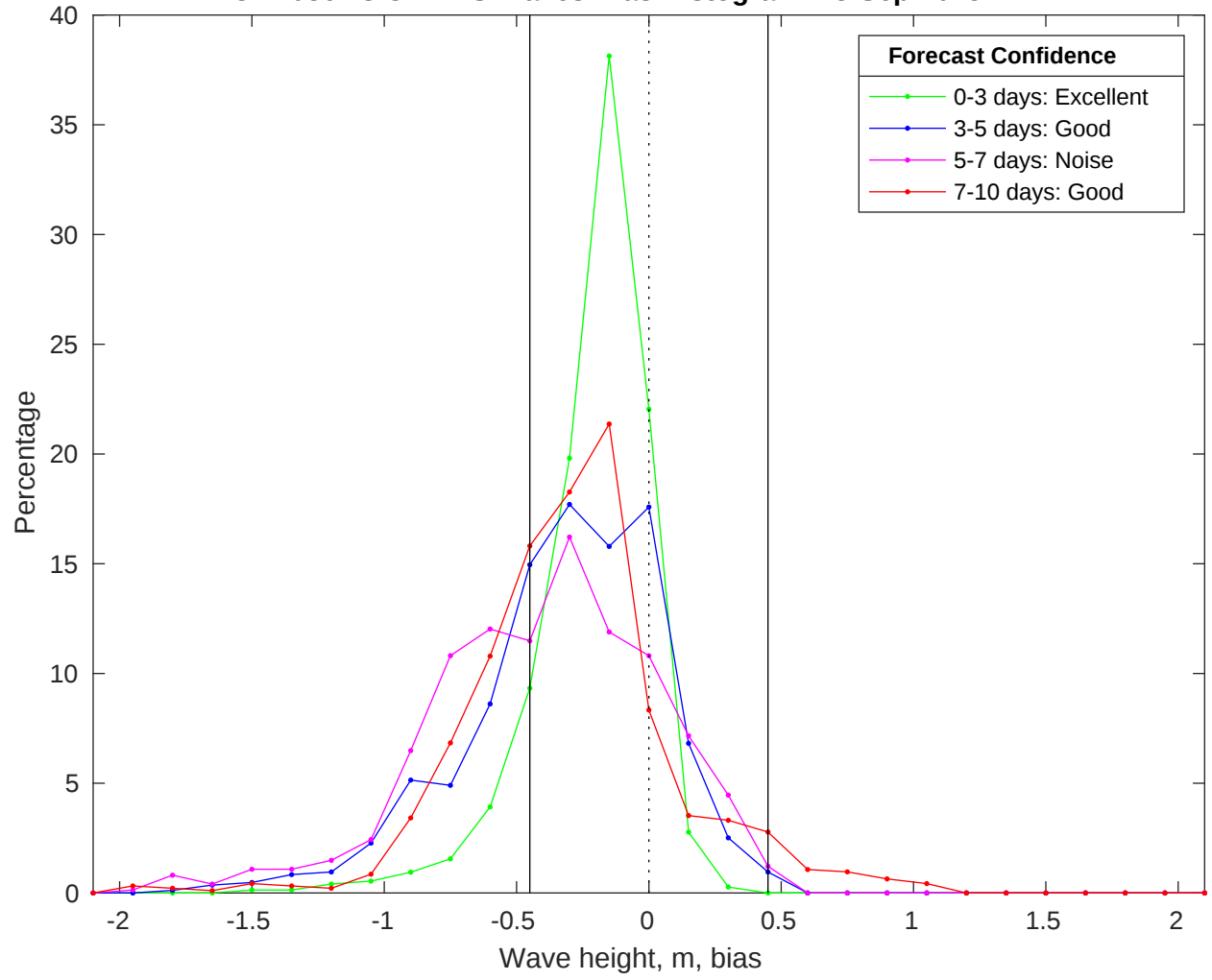
NDBC 42036 vs CMEMS Waves Bias Histogram: 23-Sep-2025
