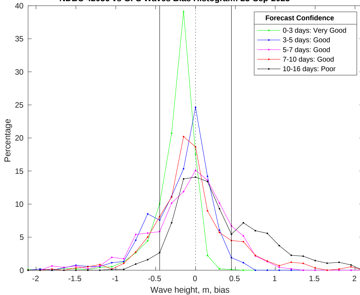
NDBC 42036 vs GFS Waves Bias Histogram: 23-Sep-2025
