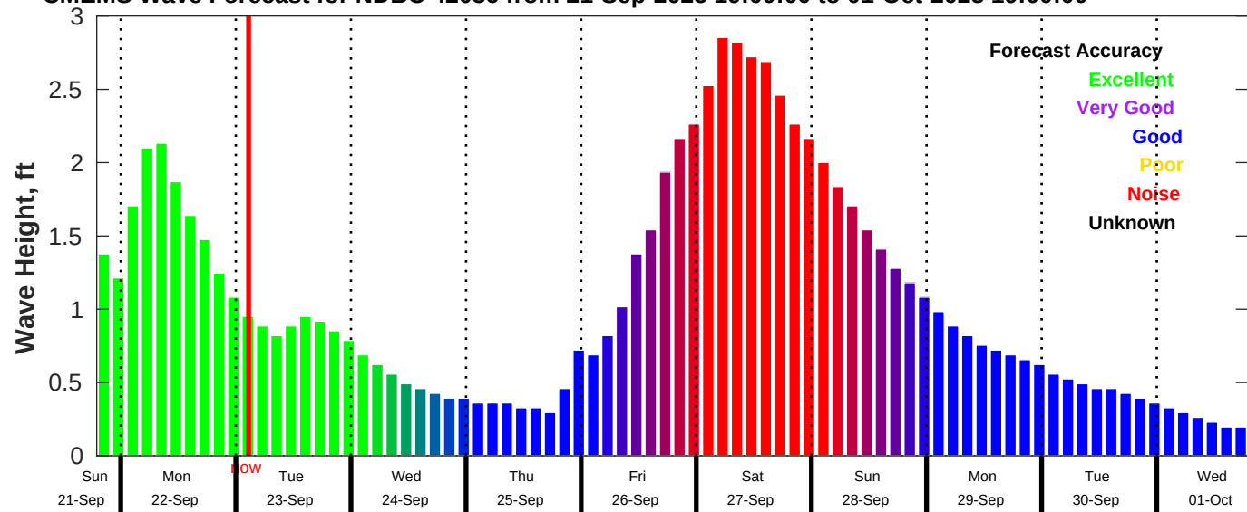
CMEMS Wave Forecast for NDBC 42036 from 21-Sep-2025 19:00:00 to 01-Oct-2025 19:00:00
