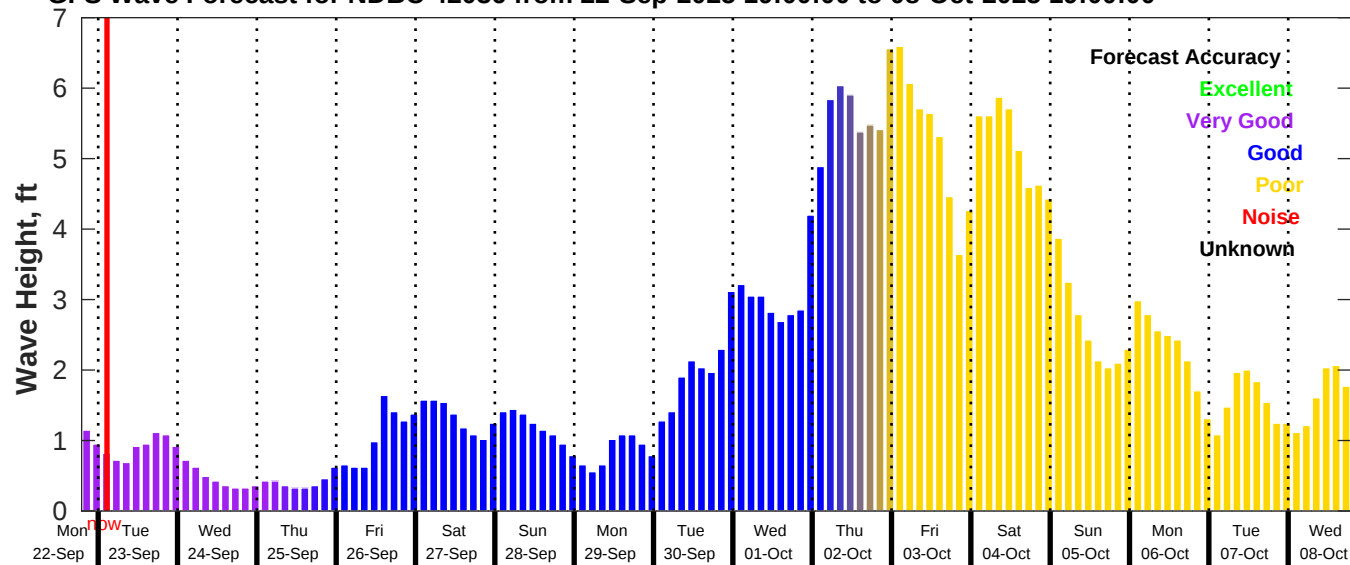
GFS Wave Forecast for NDBC 42036 from 22-Sep-2025 19:00:00 to 08-Oct-2025 19:00:00
