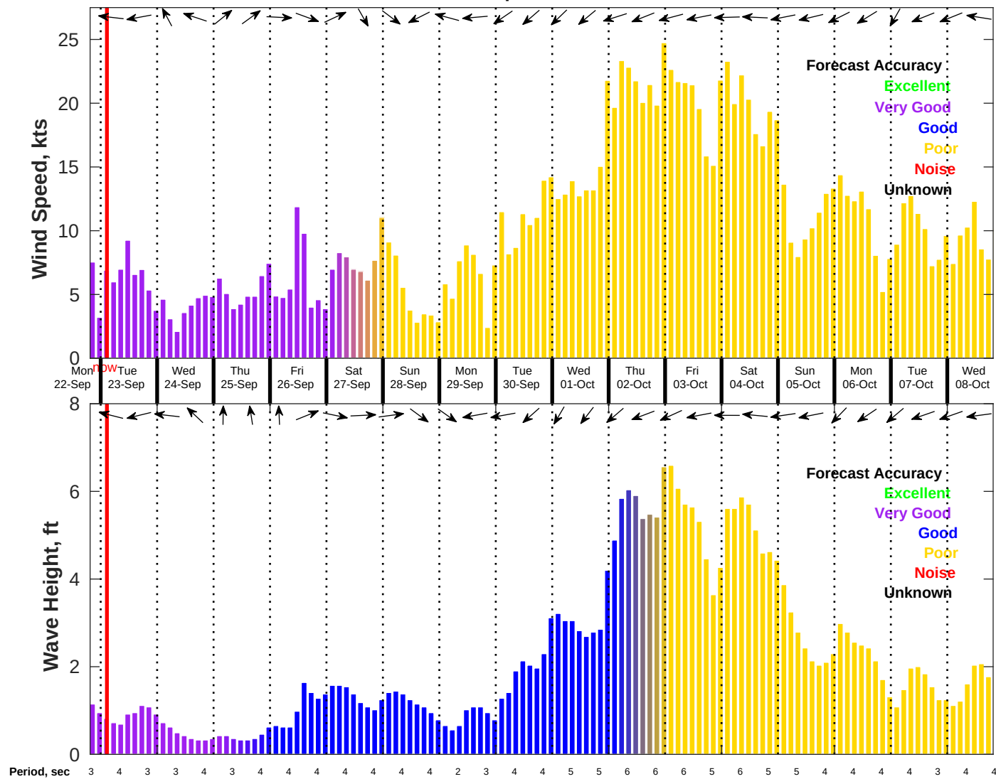
Wind & Wave Forecast for NDBC 42036 from 22-Sep-2025 19:00:00 to 08-Oct-2025 19:00:00
