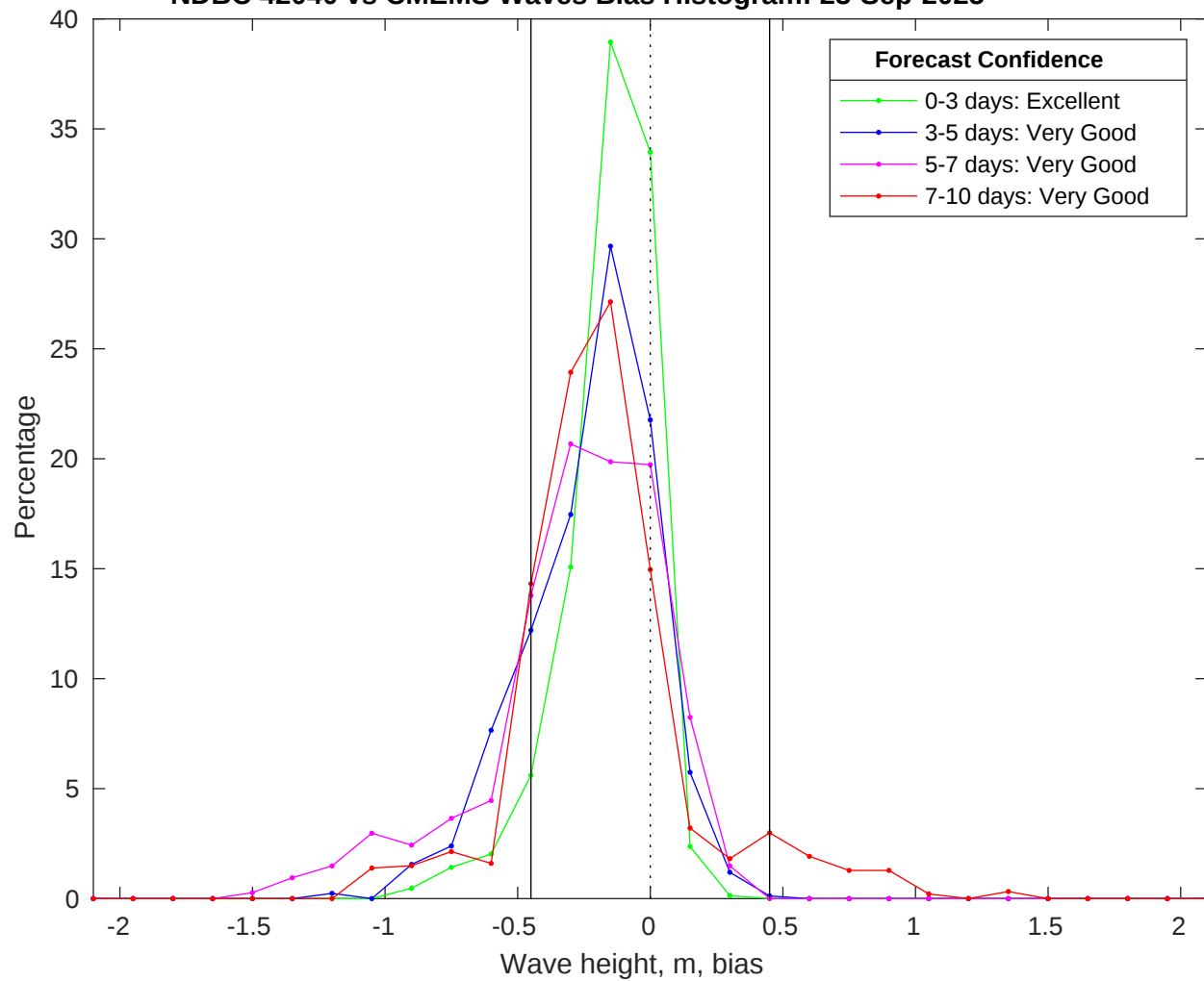
NDBC 42040 vs CMEMS Waves Bias Histogram: 23-Sep-2025
