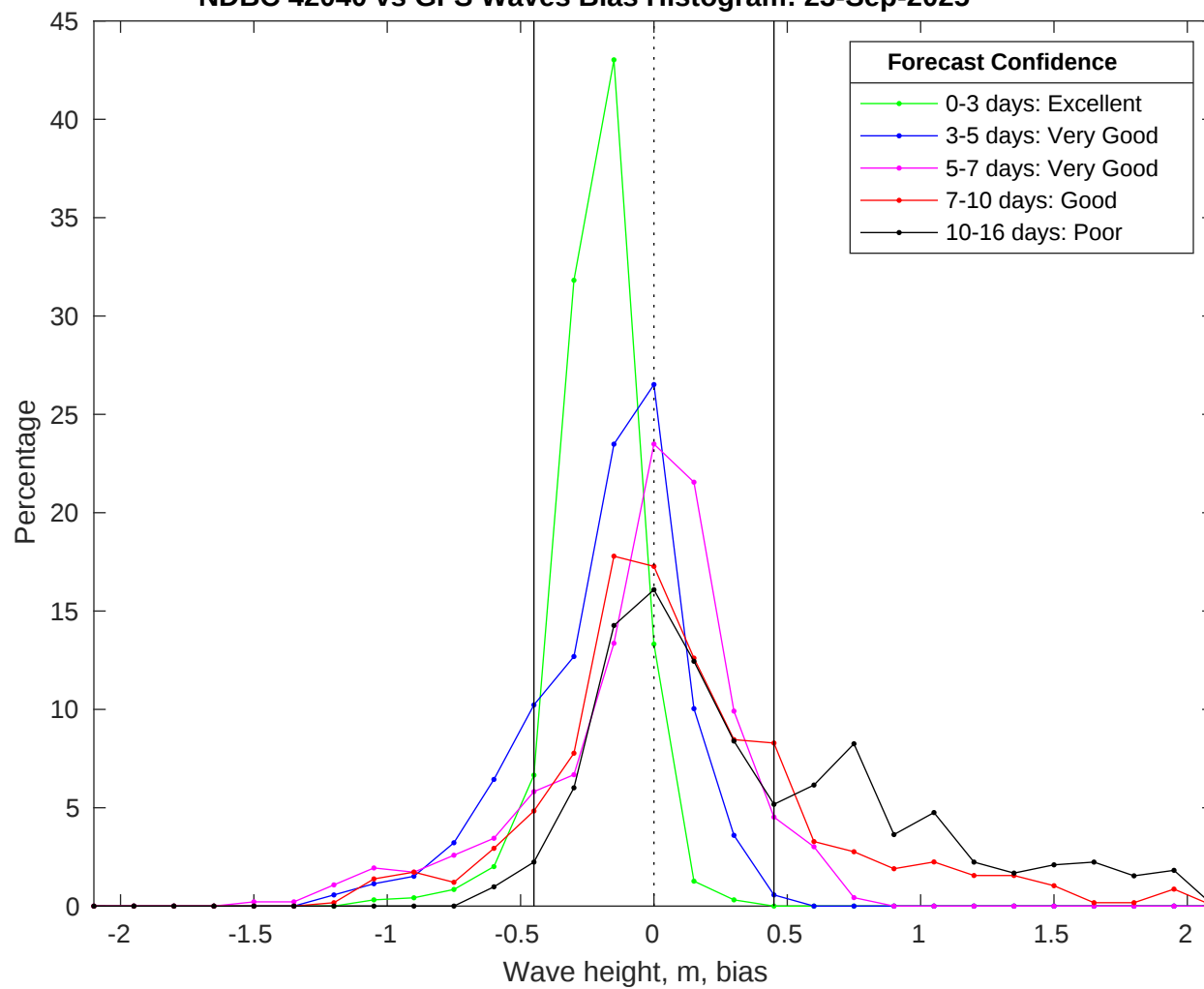
NDBC 42040 vs GFS Waves Bias Histogram: 23-Sep-2025
