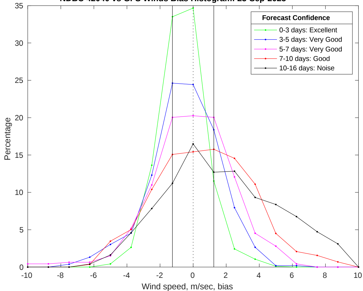
NDBC 42040 vs GFS Winds Bias Histogram: 23-Sep-2025
