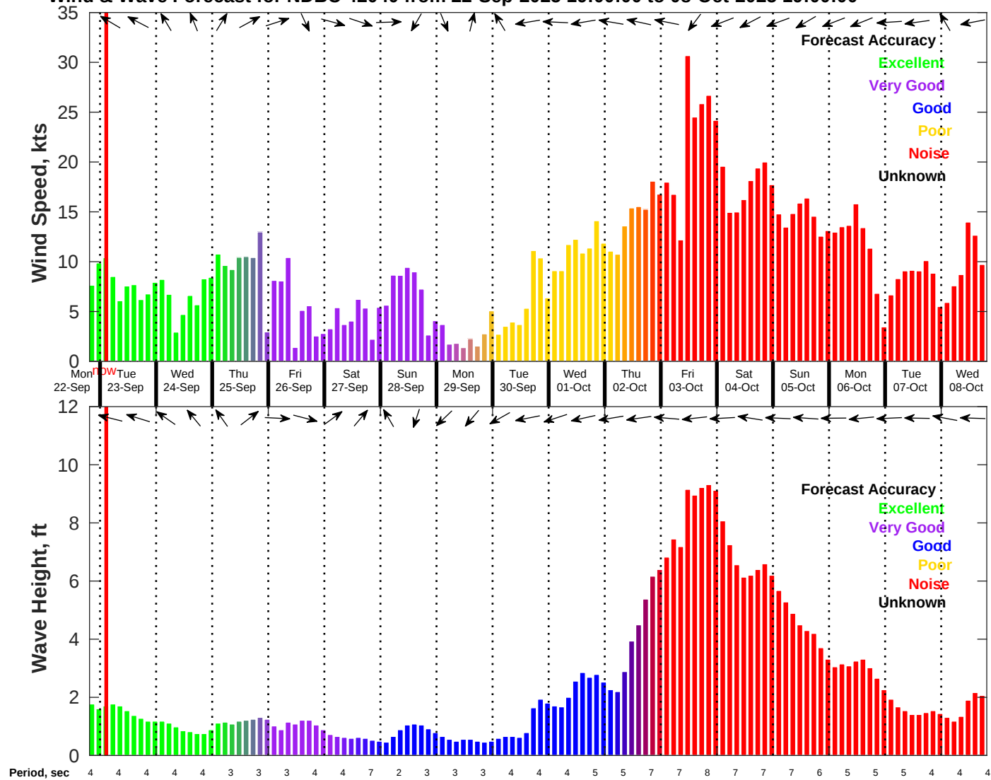
Wind & Wave Forecast for NDBC 42040 from 22-Sep-2025 19:00:00 to 08-Oct-2025 19:00:00
