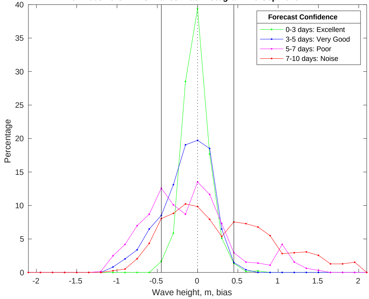
NDBC 44008 vs CMEMS Waves Bias Histogram: 23-Sep-2025
