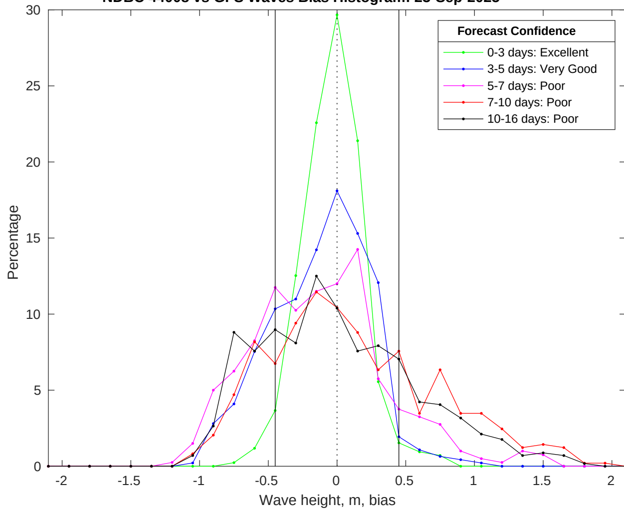
NDBC 44008 vs GFS Waves Bias Histogram: 23-Sep-2025
