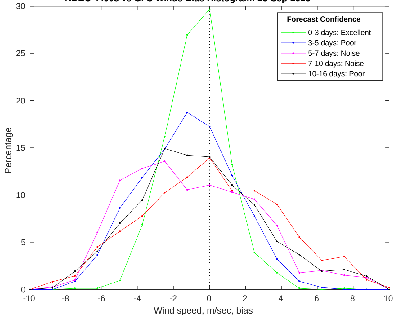
NDBC 44008 vs GFS Winds Bias Histogram: 23-Sep-2025
