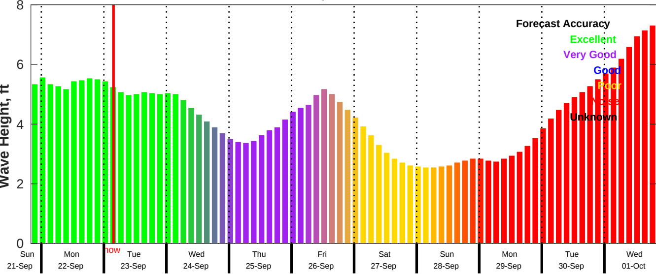
CMEMS Wave Forecast for NDBC 44008 from 21-Sep-2025 20:00:00 to 01-Oct-2025 20:00:00
