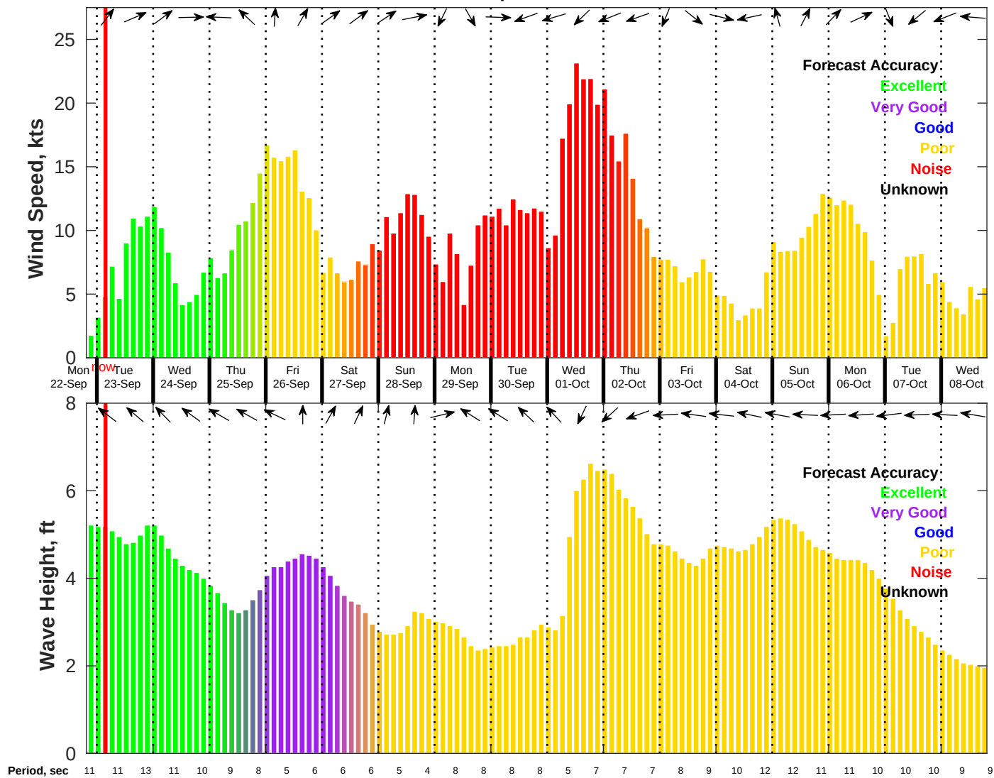
Wind & Wave Forecast for NDBC 44008 from 22-Sep-2025 20:00:00 to 08-Oct-2025 20:00:00
